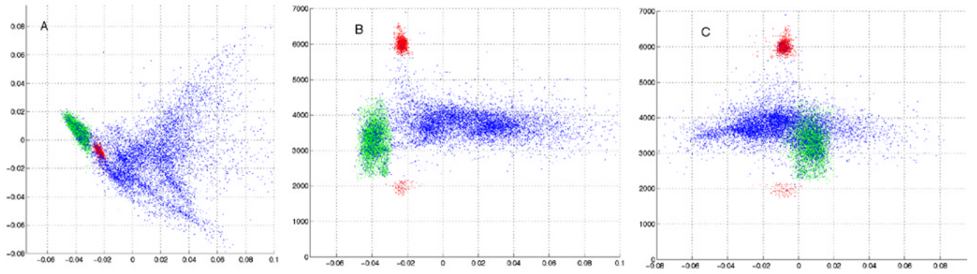
Fig. 8. Conical scatterplot of Fig. 6 converted to a cylindrical scatterplot. The offset values of the second and third PCs as given in (2) and (3) are normalized by the first PC. (A) P_2 - P_3 plane. (B) P_2 - P_1 plane. (C) P_3 - P_1 plane. All points with the same spectral character but different intensities should appear at the same cylindrical radius, but at different vertical positions.
