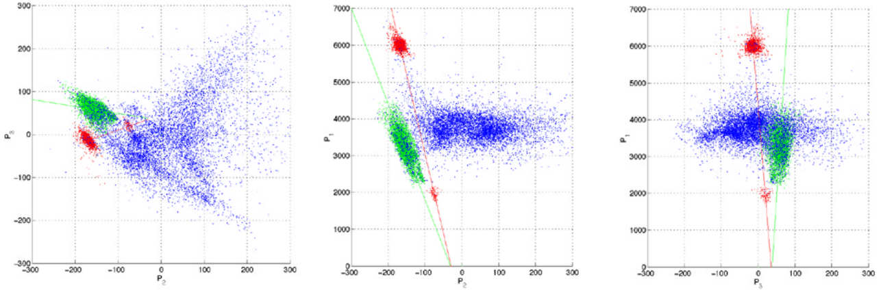
Fig. 6. Scatterplot of the data from Fig. 5 projected onto the three principal planes of the 3-D data cone. (A) P_2 - P_3 plane. (B) P_2 - P_1 plane. (C) P_3 - P_1 plane. The pixels highlighted in red were from one of two regions: the bright pixels were from the playa at the lower right of the image, and the dark pixels were from the dark region just left of center in the image. The pixels highlighted in green were from the mountainous region in the upper right of the image. The two groups of highlighted pixels were assumed to lie near lines emanating from the unknown origin of the conical data space. The red and green lines represent least-squares fits to the highlighted data clouds, and their near intersection at P_1 = 0 provides an estimate for the location of the origin. The geometric mean of the data cloud is at P_1 = 3716 , P_2 = -0.604 , P_3 = 1.25 . In panel (C), the red and green clusters are located behind the majority of the data cloud, as can be seen from the top view in panel (A).
