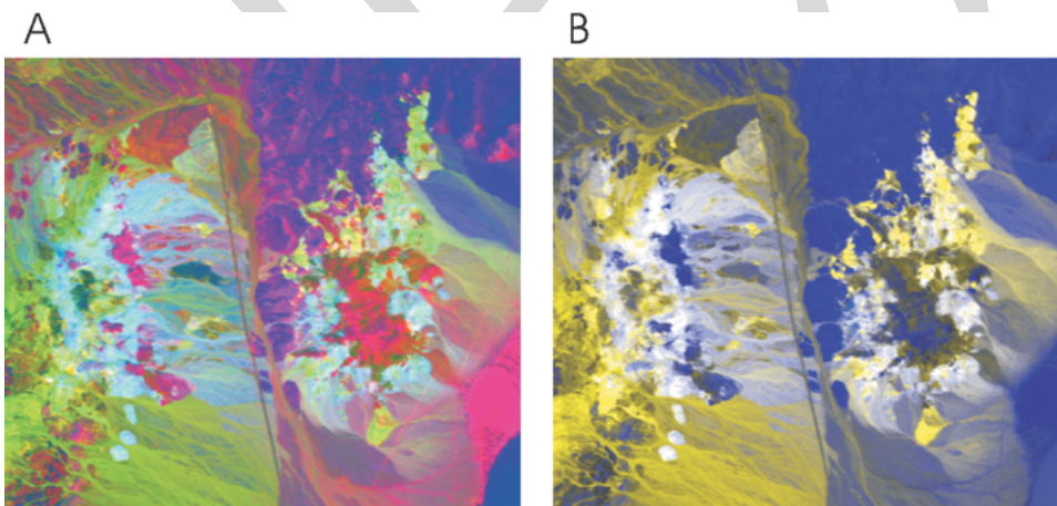
Fig. 5. Pseudocolor representations obtained by conventional mappings of PC image data into (R, G, B) space. (A) (P_1, P_2, P_3) \rightarrow (R, G, B) . (B) (P_2, P_2, P_3) \rightarrow (R, G, B) .
