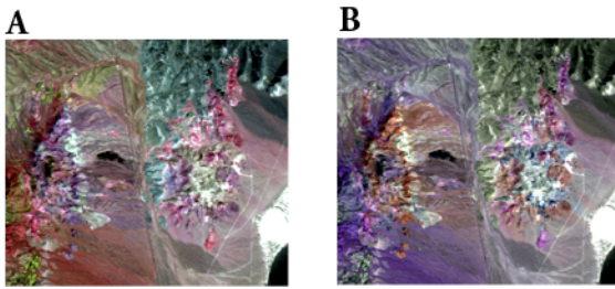
Fig. 1. Two common mapping strategies for spectral data. (A) Three widely spaced bands are chosen in hopes that they are minimally correlated \lambda = (2.101 \mu\text{m}, 2.2008 \mu\text{m}, 2.13402 \mu\text{m}) . (B) Three specific bands are chosen to highlight a particular spectral feature \lambda = (2.2307 \mu\text{m}, 2.2008 \mu\text{m}, 2.1309 \mu\text{m}) . It is expected that the mineral kaolinite will appear as magenta in panel (B), as the green intensity in the RGB image is chosen to lie at the bottom of a kaolinite absorption feature.
