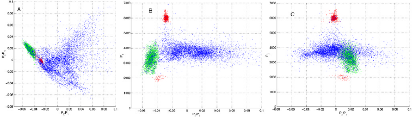
Fig. 7. Conical data normalized by P_1 without first shifting the origin. (A) P_2 - P_3 plane. (B) P_2 - P_1 plane. (C) P_3 - P_1 plane. There is a slight tilt to the data that will affect the opponent color mapping strategy presented in Section IV.
