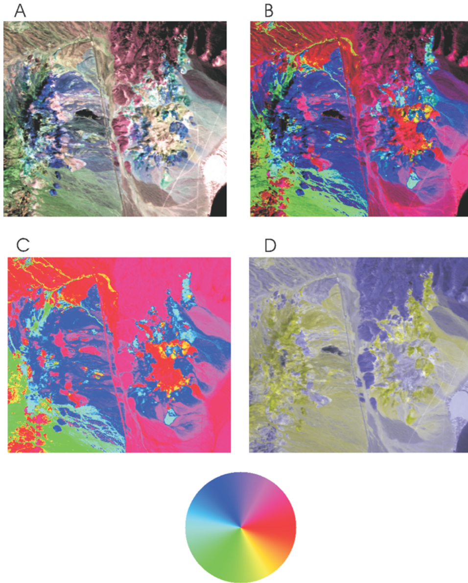
Fig. 9. Four mappings which translate the first three PC images into the (H, S, V) color space. (A) Full implementation of (5) with saturation amplified so that the maximum value of S in the image is unity. (B) Suppression of saturation. Each pixel is fully saturated, but the first and third equations in (5) are still employed. (C) Only the hue is mapped. (D) A specialized mapping designed to locate regions of an image that are similar or dissimilar to a particular spectral signature. In this case, yellow pixels have a positive second PC, blue pixels negative. The third PC information is suppressed.
