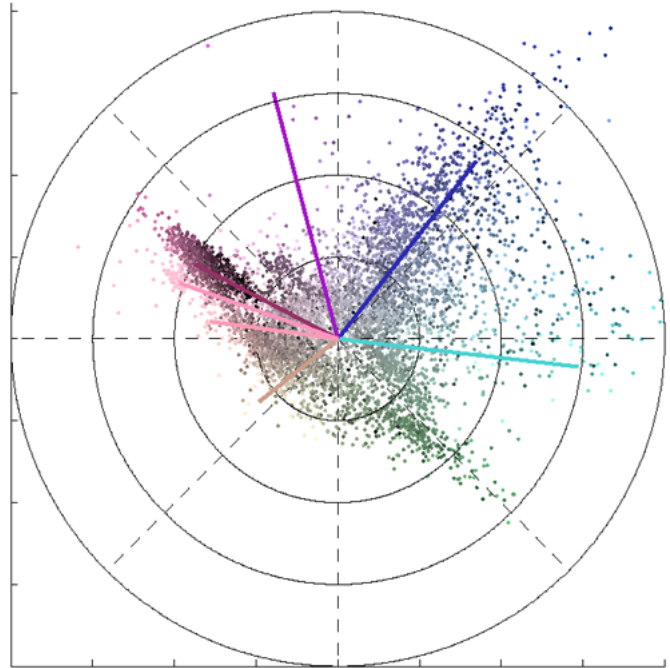
Fig. 11. Scatterplot representation in the P_2 - P_3 plane with the point corresponding to each pixel colored with the same (H, S, V) triple as in the image in Fig. 9(A). Only one out of every twenty pixels is plotted here to aid in viewing the result. Unsaturated (gray) pixels are those near the origin, and particular hues radiate outwards. The lines are drawn from the origin to the mean of the classes in Table I. Note that the means each have a different value of P_1 which does not appear in this figure, since P_1 is orthogonal to this projection.
