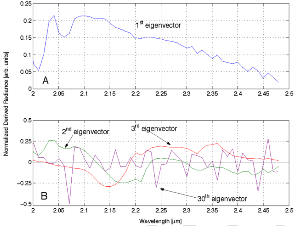
Fig. 3. First three eigenvectors of the covariance matrix for the image depicted in Fig. 1. Note that the first eigenvector is all positive, and the second and third have similar spectral frequency variation, though they are orthogonal. The 30th eigenvector has much more spectral variability, and the variance in the corresponding PC image is 1000 times lower than in the second and third PC images. All eigenvectors are normalized so that \|\mathbf{v}\|_2 = 1 . The second and third eigenvectors have properties of “out of phase” functions like sine and cosine, as the extrema of the second PC tend to line up with zero-crossings of the third PC and vice-versa.
