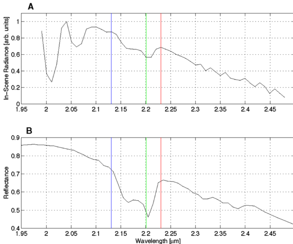
Fig. 2. (A) Representative radiance spectrum of kaolinite taken from a region in the image known to contain that mineral on the surface. (B) Reflectance of Kaolinite from the U.S. Geological Survey spectral library (provided with ENVI). The vertical lines give the spectral locations corresponding to the red, green, and blue intensities in panel (B) of Fig. 1.
