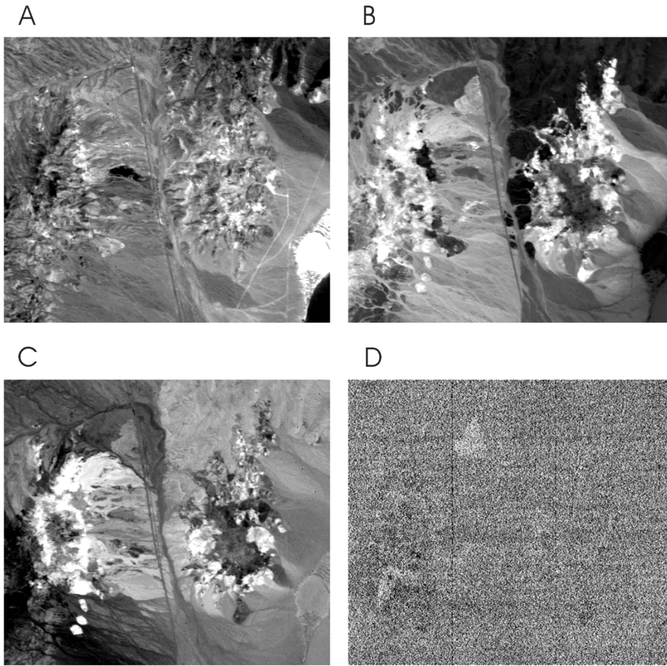
Fig. 4. PC image numbers 1, 2, 3, and 30. The high spatial frequency information corresponding to geography is represented in the first PC image [panel (A)], while lower spatial frequency information corresponding to classification information is represented in the second and third PC images [panels (B) and (C)]. The spatial frequency content of panels (B) and (C) are similar, as are the overall spectral shapes of the second and third PCs. Panel (D) contains the 30th PC image. Notice that it has little low spatial frequency structure, as its eigenvalue indicates. There is little grouping information available in this principal component, as there is little spectral clustering in the corresponding eigenvector in Fig. 3.
